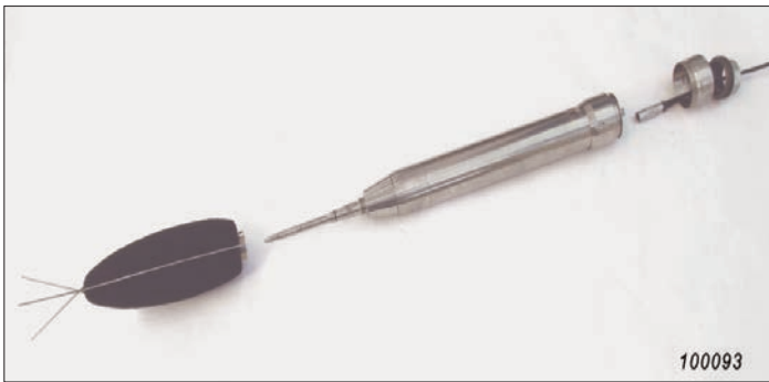
Fig. 6 Weatherproof Microphone Type 4184-A with adaptor for easy fitting onto the top of a standard water pipe
